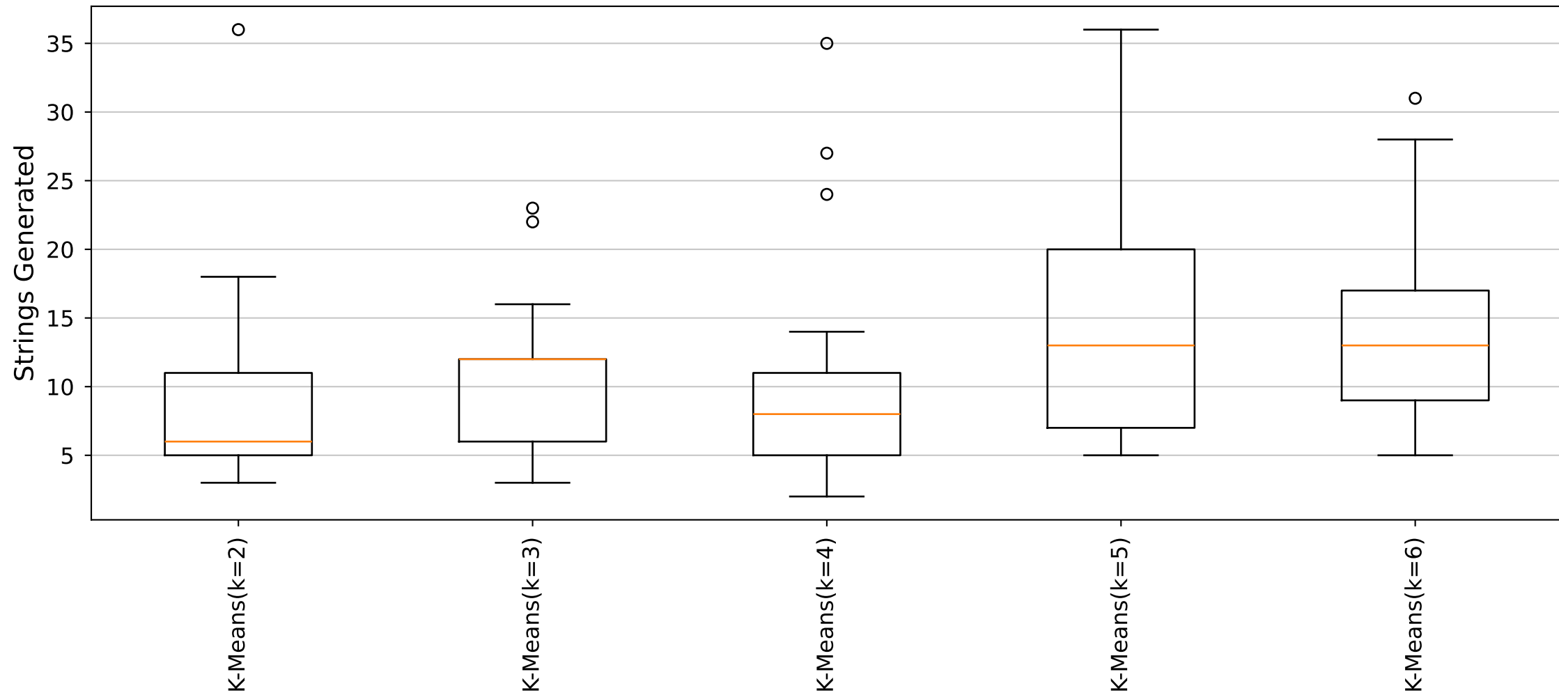
YARA Rules Strings Generated Distribution (Cluster24_Size6 dataset)
